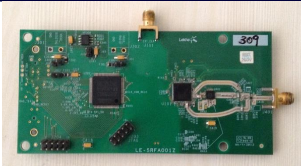
Wideband RF Card
